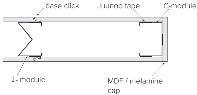
horizontal section
